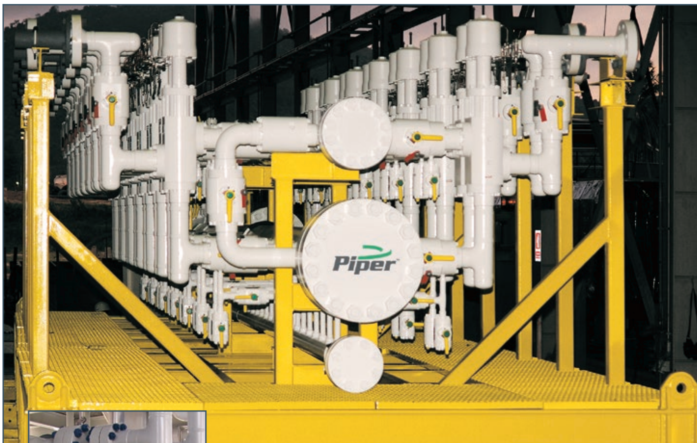
28-Slot Offshore Production Manifold utilizing compact manifold ball valves, check valves and poppet diverter valves.
