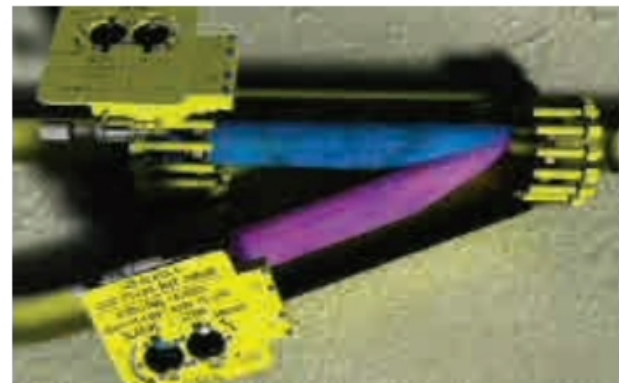
Dual Director Sleeve Rotated Permitting Bi-Directional Pigging in the Lateral Line.
