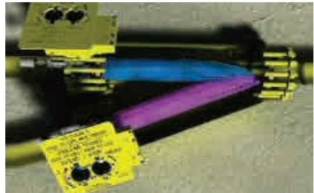
Dual Director Sleeve Rotated Permitting Bi-Directional Pigging In the Main Line.
